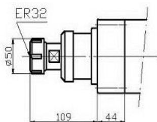
FD67SS-85-ER32
