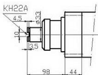
FD67SS-85-KH22A
